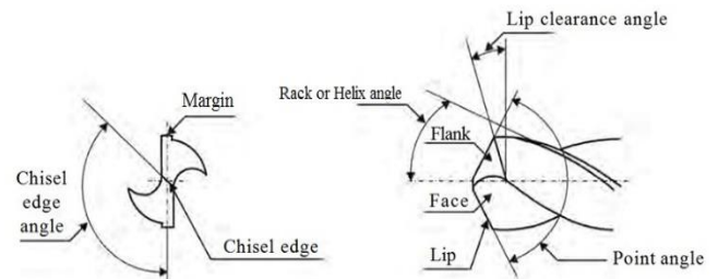
Fig.5: Drill nomenclature
