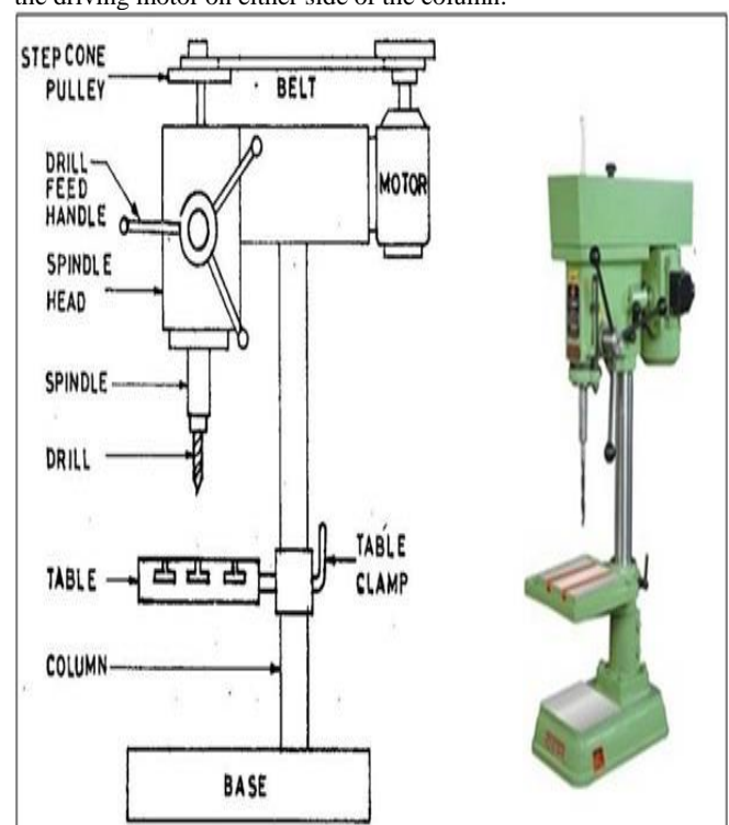
Fig.1: Drilling machine
