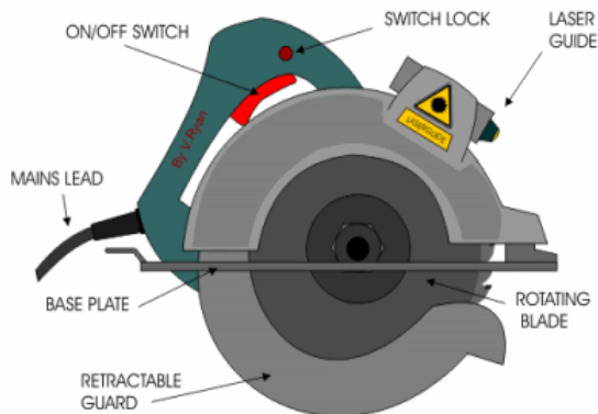
Fig. 10: Circular saw
