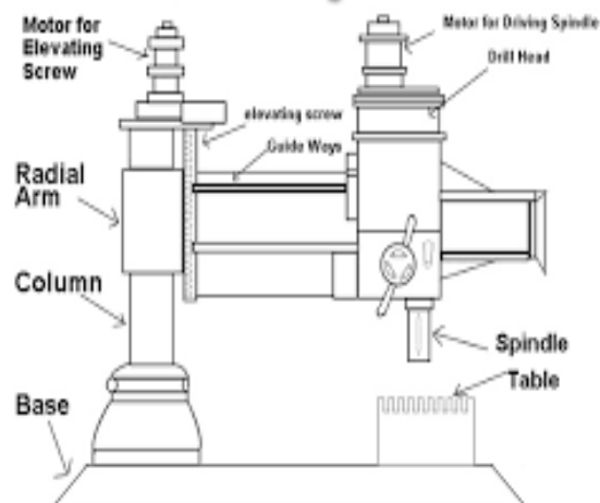
Fig.3: Radial drilling machine
