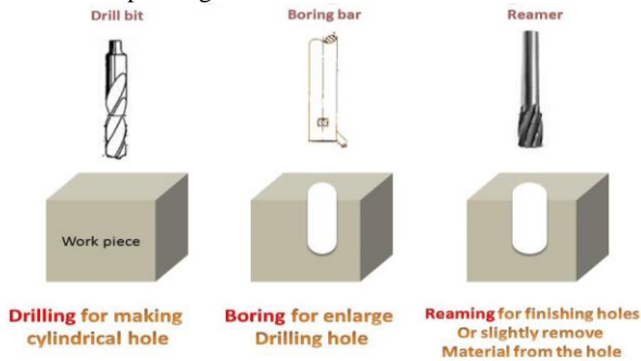
Fig.7: Drilling, boring and reaming
