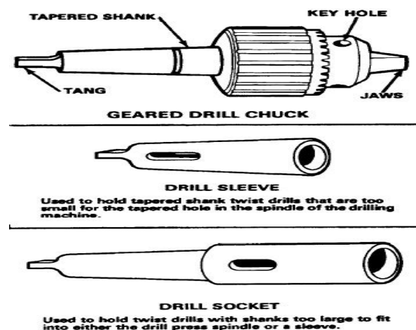
Fig.6: Tool holding devices
